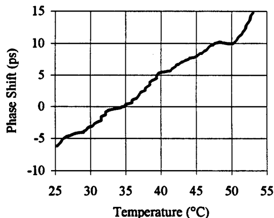
Figure 7. Phase-temperature coefficients
