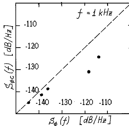
Figure 6. Comparison of power spectral density measured in oscillator S_\phi(f) with the one calculated on the base of in-bridge measurement S_{\phi c}(f)
