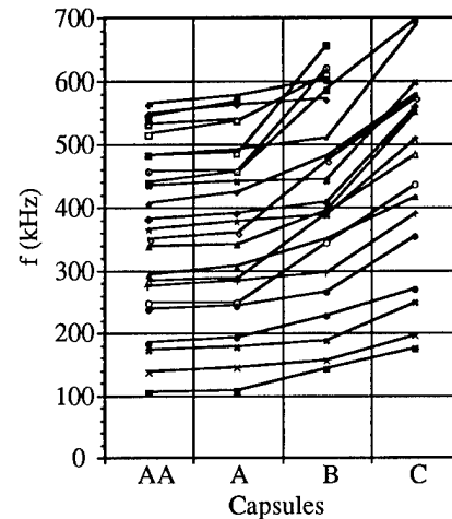
Fig.15 Mode charts for capsules.
