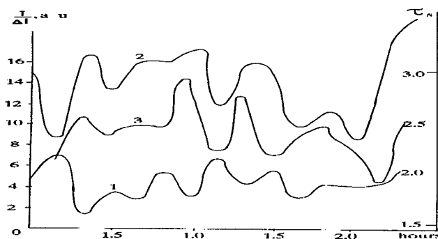
Fig.8. I a.u. for non-equilibrium desorption of H 2 O-molecules (1) and OH (2) from PTFE surface and \tau_s within a storage box (3) vs experimental time; T = 293\text{K} ; P = 10^{-5}\text{Torr} ; F = 2.5 \times 10^{14}\text{ cm}^{-2}\text{s}^{-1} ; P_{\text{H}_2\text{O}} = 20\text{ Torr} .
