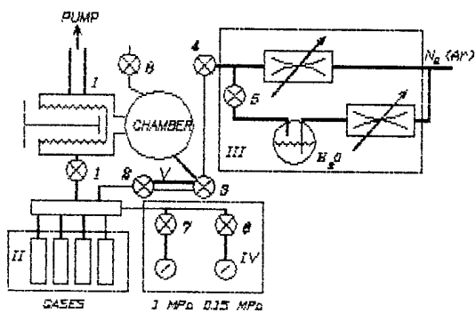
1, 2, 3, 4, 5, 6, 7, 8 - valves; I - faucet; II - balloons with gases; III - insuffle system; IV - manometers; V - by pass volume. Relation volume of by pass to chamber is equal to 1:300. Fig. 4 Block diagram of measurement gas sensitivity.
