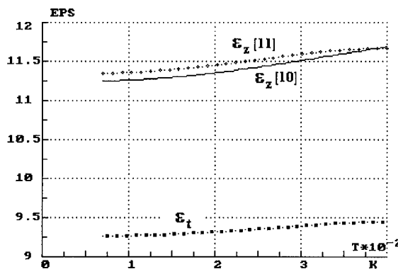
Fig.1. Sapphite relative permittivity components versus temperature.
