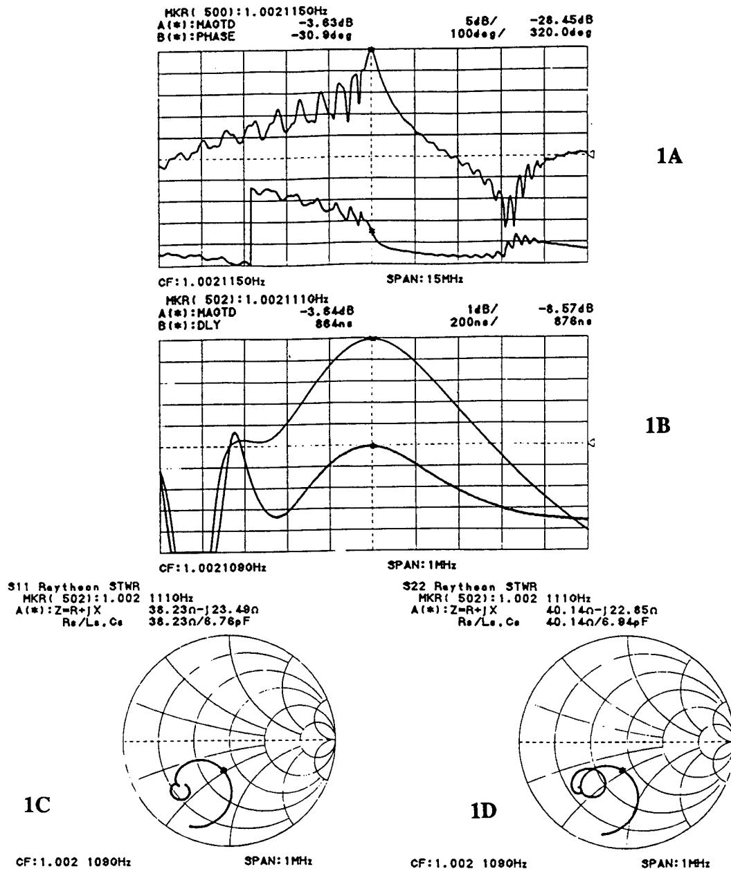
Fig. 1. Characteristics of a single mode high-Q device realized at Raytheon:
