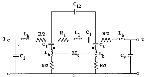
Figure 4. Surface Acoustic Wave Resonator Model.
