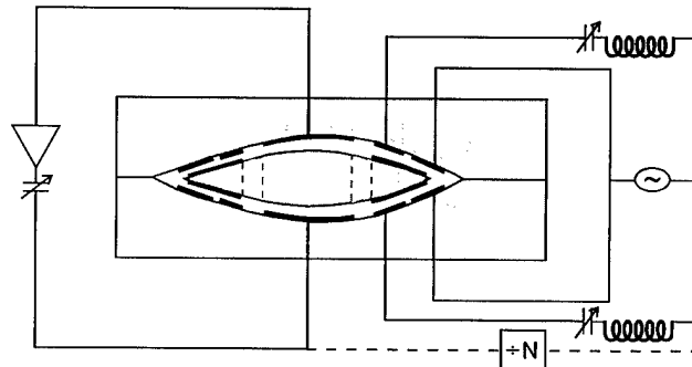
Fig. 10 One approach to combine levitation with the BVA style resonator. From [84].
