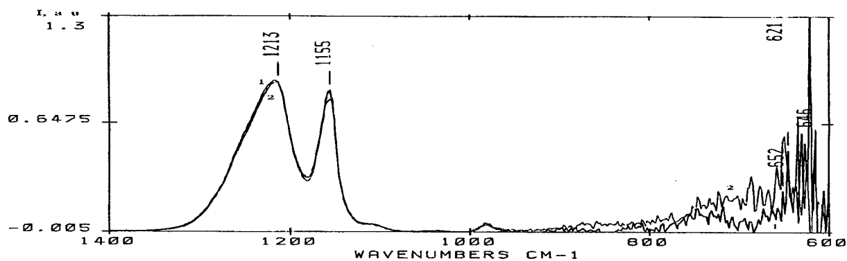
Fig.11. FTIR spectra for FBCC: initial (1), after treatment in a low temperature CF plasma (2), after e-irradiation in Leybold Hereaus surface analyzer at 10^{-8} Torr, U = 3\text{kV} , J = (1-10)\mu\text{A} , D = 10^6 - 10^8 rad.
