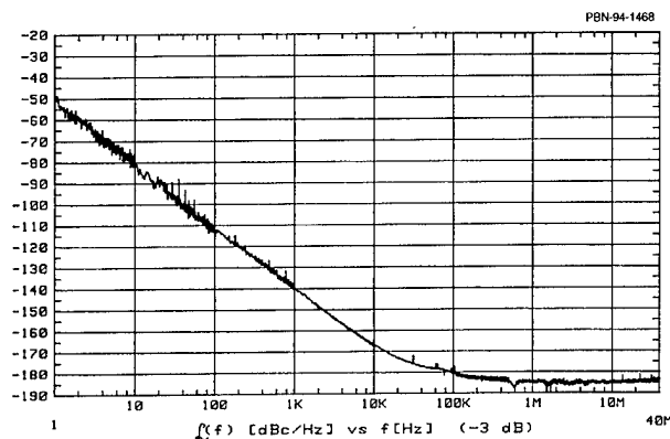
Figure 4(b). Measured phase noise for one prototype extremely low noise AQP SAW resonator hybrid circuit oscillator after system floor correction has been made, and 3 dB has been subtracted under the assumption that the two oscillators are identical.
