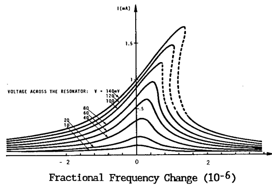
Fig. 3 Non-linear resonance as a function of RF drive for a 5 MHz AT-cut resonator. From [22].
