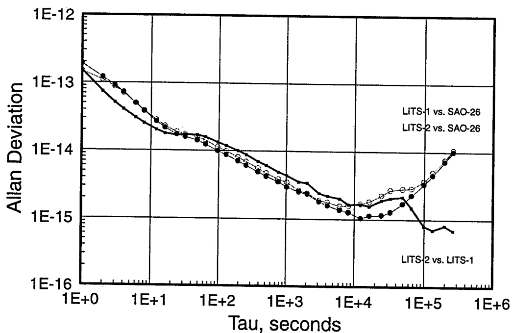
Figure 3: Nine day comparison between the \text{Hg}^+ trapped ion standards LITS-2 and LITS-1. Both standards are also compared to the H-maser SAO-26 over the same time interval.
