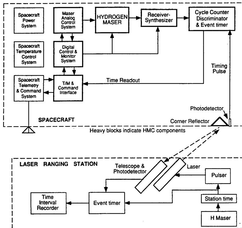
Fig. 2. Block diagram of major HMC experiment components
