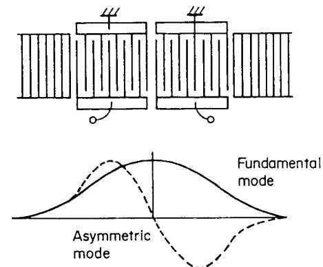
Fig. 5. Arrangement of IDT for the conventional 2-port resonator and its charge distributions of fundamental and spurious asymmetric modes. (From S. Matsumura et al. [24])
