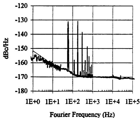
Figure 5. Phase noise of isolation amplifier
