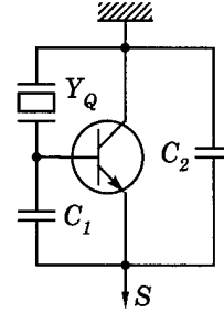
Fig. 6 : Simplified form of a Colpitts oscillator
