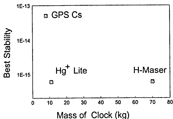
Figure 2. A summary of clock frequency stability vs. clock mass for three space based frequency standards discussed in this paper. The proposed Hg + LITE can supply stability of a maser in a total package with mass comparable to the current day GPS Cs standards.
