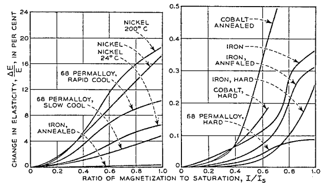
Fig. 6 : Change in Young's modulus with magnetization (after [9]).
