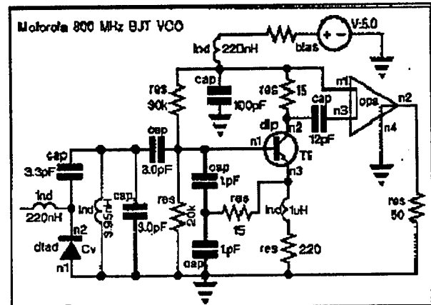
Fig. 9 - Colpitts Oscillator which uses RF feedback
