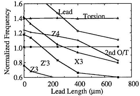
Fig.17 Mode charts for lead length.
