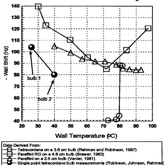
Figure 4: This figure presents ^{87}\text{Rb} wall shift data for n-tetracontane and for Paraffint as measured by different investigators over the last 30 years.
