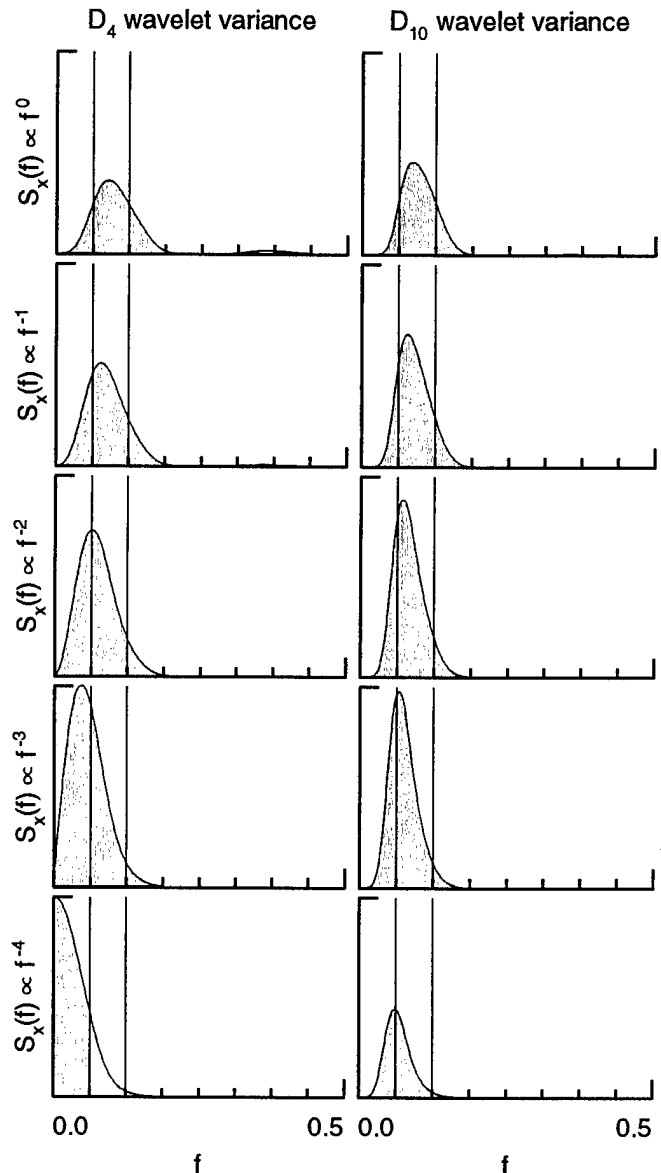
Fig. 3. Modulus squared of the transfer function for the D_4 wavelet variance (left-hand column) and the D_{10} wavelet variance (right-hand column) times the same set of power-law spectra shown in Fig. 2. The integrals of the shaded areas yield the D_4 or D_{10} wavelet variance for scale \tau = 4 .
