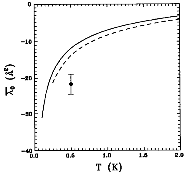
Figure 4: A comparison of the spin-exchange frequency shift cross section \bar{\lambda}_0 measured as outlined in this article with the most sophisticated theoretical calculation of this parameter to date (full curve) [6, 7]. An earlier calculation of \bar{\lambda}_0 (dashed curve) [26] based on less accurate potentials is included to give the reader a feeling for the sensitivity of the calculated result to the details of the potentials.
