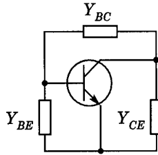
Fig. 2 : \Pi -reduced form of an oscillator
