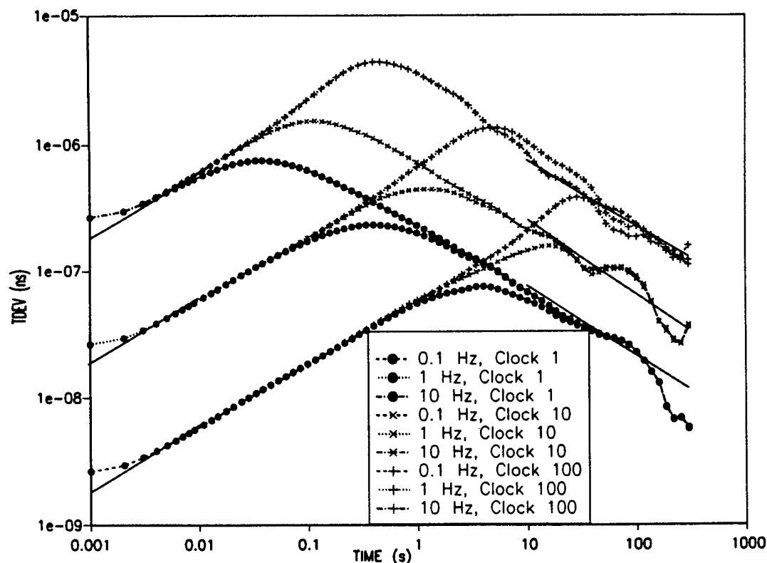
Figure 3. TDEV Due to Phase Detector White Phase Noise in Chain of Clocks ( c2 = 1.0\text{e-}17 \text{ rad}^2/\text{Hz} )
