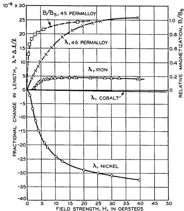
Fig. 8 : Magnetostriction of some ferromagnetic materials [9].
