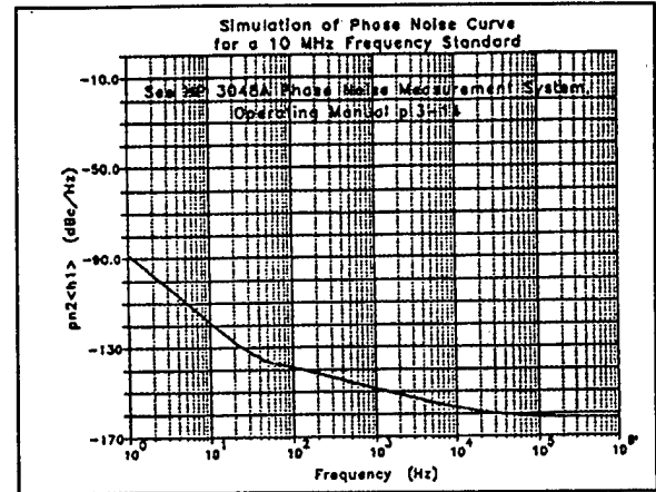
Fig. 8 - Simulated phase noise of the oscillator shown in Fig. 6
