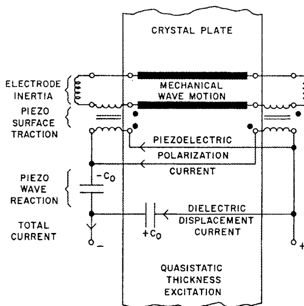
Fig. 1. Exact electrical equivalent network for a single thickness mode driven by thickness-field excitation in a laterally unbounded piezoelectric resonator.
