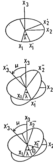
Fig. 1 Coordinate system used to define SAW propagation.
