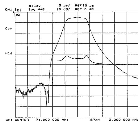
Fig. 11. Frequency response of the reversely connected SAW filter. The SAW filter has three IDTs with multielectrodes in a propagating track.
