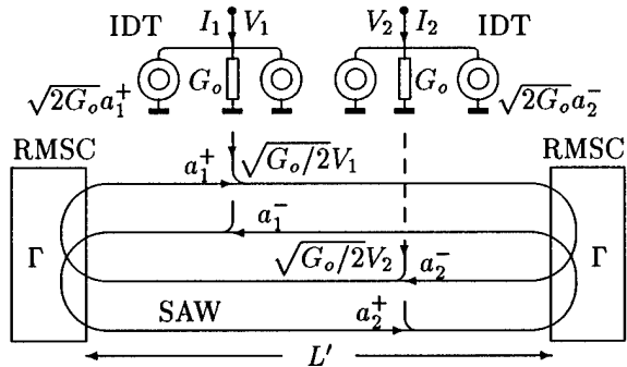
Fig.2. RMSC symmetric two-port SAW resonator. (Remark: At the second overtone frequency, r/K appearing in Eqs.(3) is twice as much. This reduces r_o - r_v , and \bar{\kappa} in Eqs.(14), thus the RMSC relative stopband, by half.)
