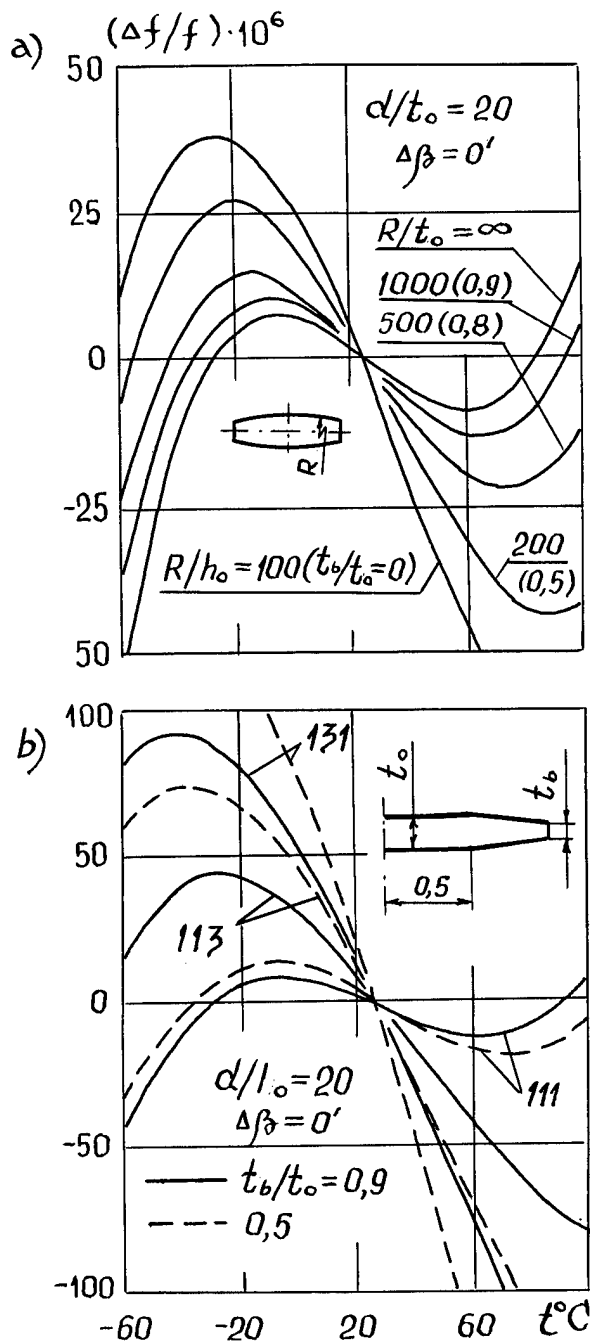
Figure 14 - Frequency- temperature characteristic of AT cut piezoelectric elements ( \beta=35.0862^\circ ) with different surface curvature: a) LPE with different radii of sphere; b) disk-type PE with bevels
