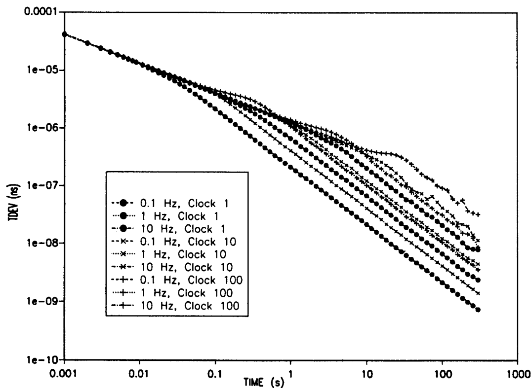
Figure 4. TDEV Due to VCO White Phase Noise in Chain of Clocks ( b2 = 3.2\text{e-}16 \text{ rad}^2/\text{Hz} )
