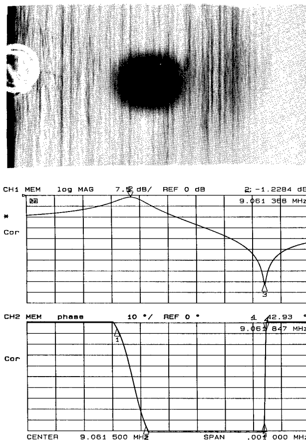
Figure 14-Topograph of the fifth overtone. The response curve shows a Q factor equal to that of the third overtone but at a frequency higher.
