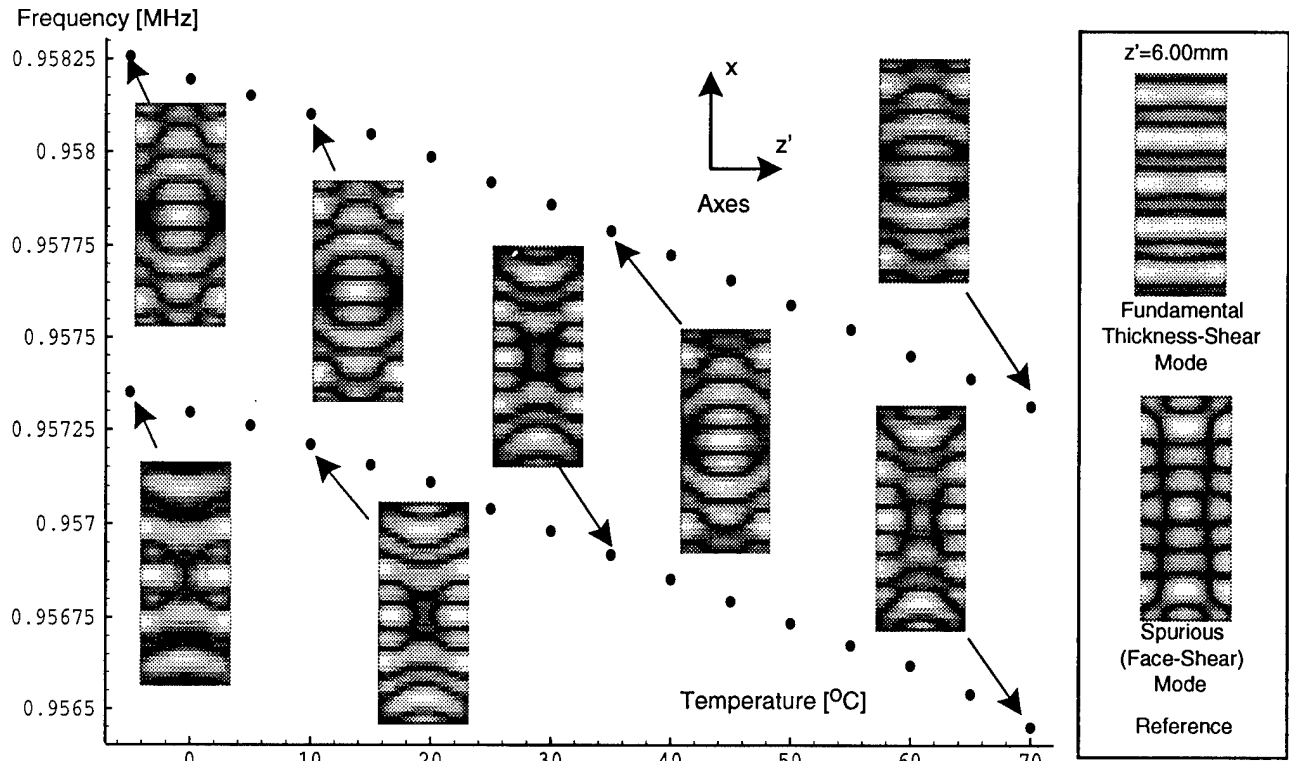
Fig.5 Experimental results for a 1MHz AT-cut quartz plate. ( 2a(x)=13.964\text{mm} , 2c(z')=5.92\text{mm} , 2b(y')=1.737\text{mm} )
