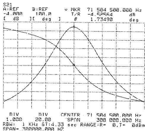
Fig.4. Narrow-band response, IDTs in parallel.
