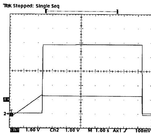
Fig. 4c Third sweep, the peculiar start-up behaviour has completely disappeared resulting in a "cured" crystal.
