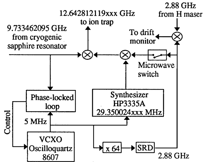
Figure 7: 12.6 GHz microwave source based on a 9.73 GHz sapphire-loaded superconducting resonator. The microwave switch is controlled by a computer to generate the Ramsey pulses. SRD = step-recovery diode.
