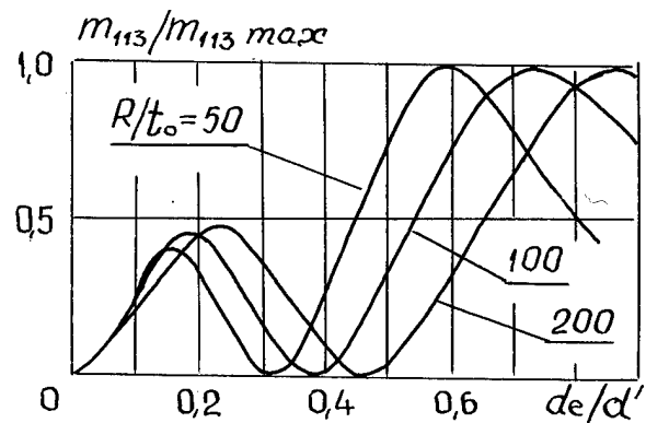
Figure 13 - Dependence of capacitance relations for anharmonic vibrations 113,131 of resonators with LPEs ( d/t_0=14 )
