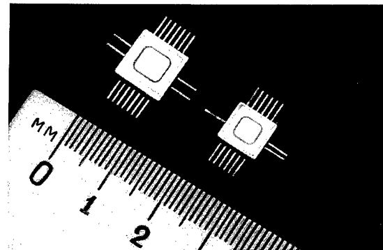
Fig. 12. Photograph of the developed ring SAW filters.
