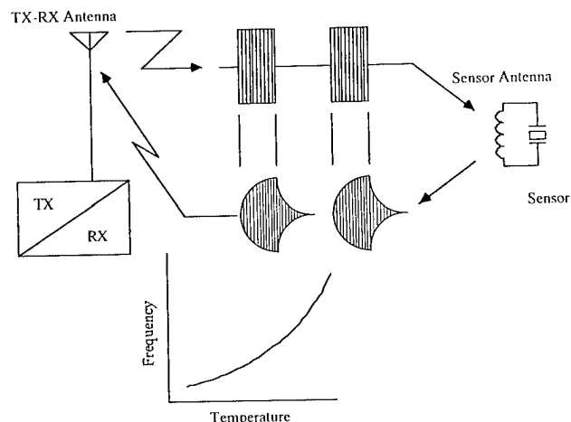
Figure 10. Principle Diagram for Wireless Echo Sensor System
