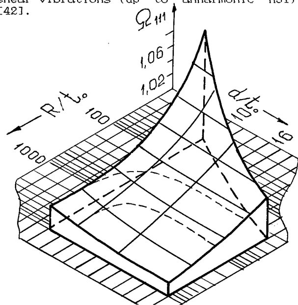
Figure 4 - Dependence of the fundamental frequency of a lens-type PE on its radius of sphere and diameter
