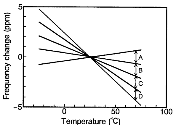
Figure 3. Range of the first order frequency temperature coefficients of the resonators used for the NS-GT-TCXO.
