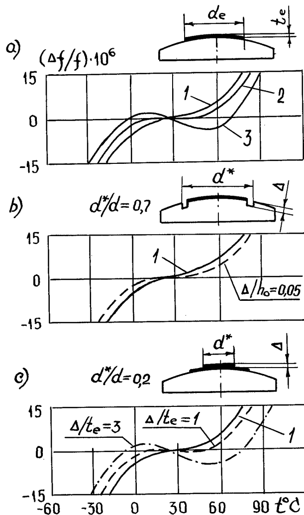
Figure 15 - Dependence of frequency-temperature characteristic on local electrode thickness changes and PE ( d/t_o=20 ; R/t_o=250 ; t_e^*=0.01 ; d_e/d=0.58 )
