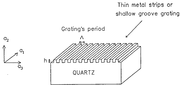
Fig. 1. Piezoelectric substrate corrugated by grooves or strips
