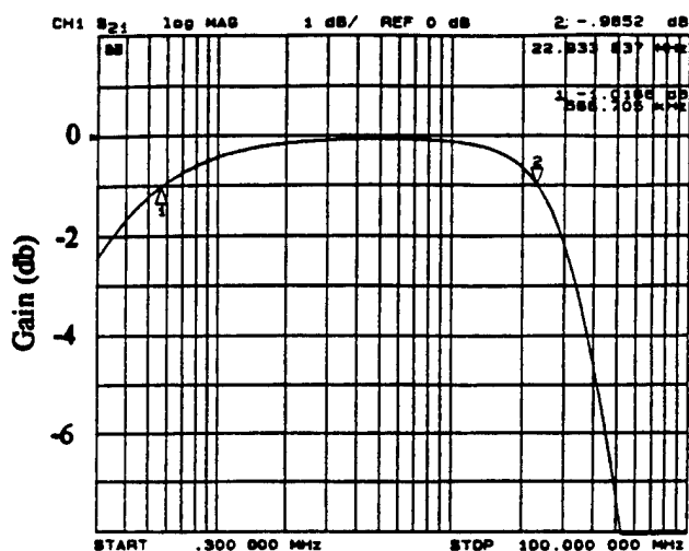
Figure 4. Gain vs. Frequency
