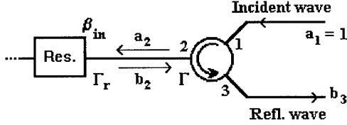
Figure 3. RWE circuitry associated with an Y-circulator.
