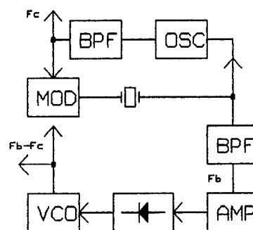
Fig.6. Dual-frequency modulation type oscillator block-diagram.
