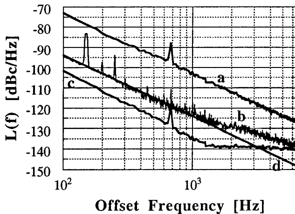
figure 12. Measured single sideband phase noise for the TE stabilized resonator-oscillator: a. open loop configuration; b. closed loop configuration; below 2 kHz we measured the noise limited due to the phase detector; above 2 kHz we measured noise due to the 8662A synthesizer; c. open loop noise divided by the loop gain; d. Oscillator noise limit due to the phase detector .
