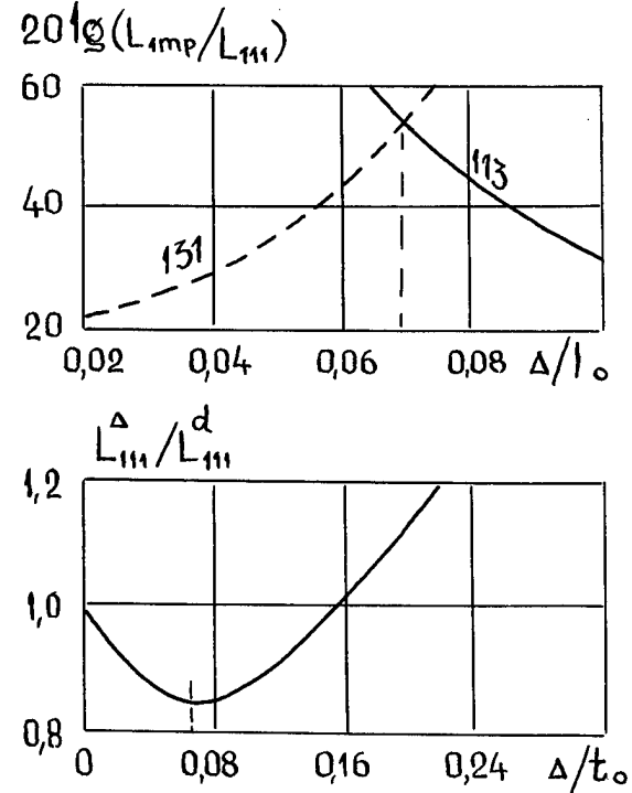
Figure 8 - Influence of PE concavity ( d/t_0=200 ; d_e/d=0.3 ; te^*=0.035 ) on the motional inductance at fundamental frequency and anharmonic vibrations
