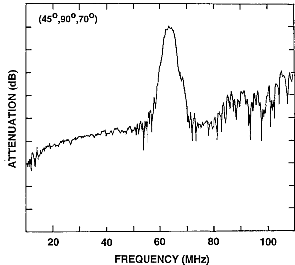
Fig. 6 Measured frequency response.
