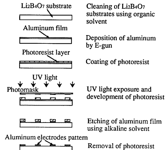
Fig. 4. Fabrication procedures of the alkaline etching process for \text{Li}_2\text{B}_4\text{O}_7 substrates.
