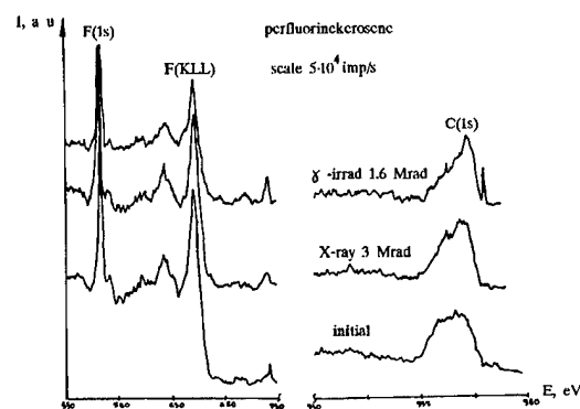
Fig.13. XPS spectra of PPC from perfluorinckerosene irradiated in the same conditions as it is indicated in Fig.12.
