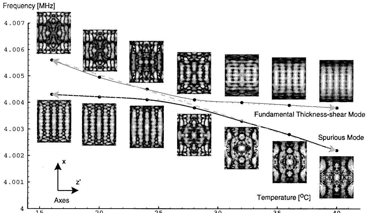
Fig.6 Experimental results for a 4MHz AT-cut quartz plate. ( 2a(x)=8.35\text{mm} , 2c(z')=7.00\text{mm} , 2b(y')=0.422\text{mm} )
