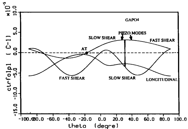
Figure 3c: FTC of the thickness modes in the Y rotated cuts of gallium phosphate.
