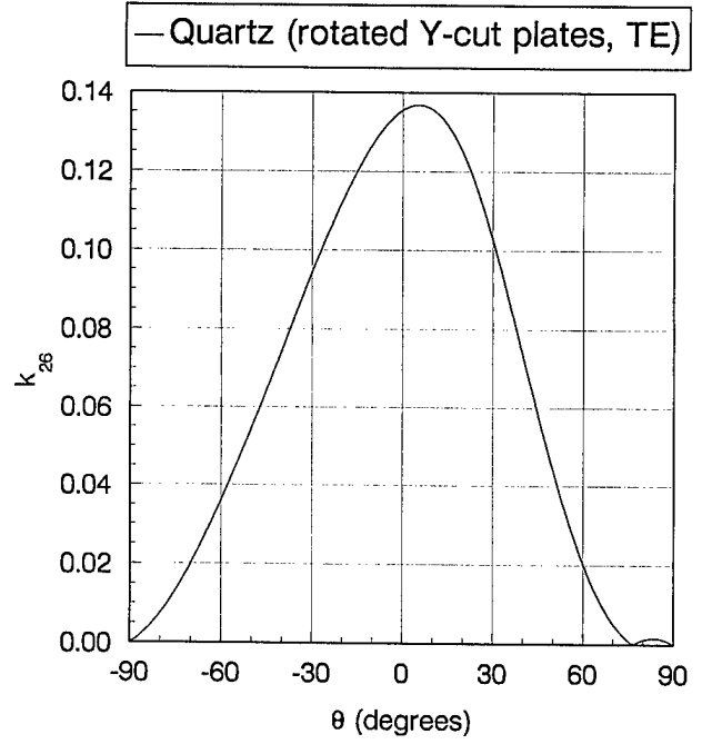
FIGURE 3. Piezoelectric coupling factor. Rotated-Y-cuts of quartz.
