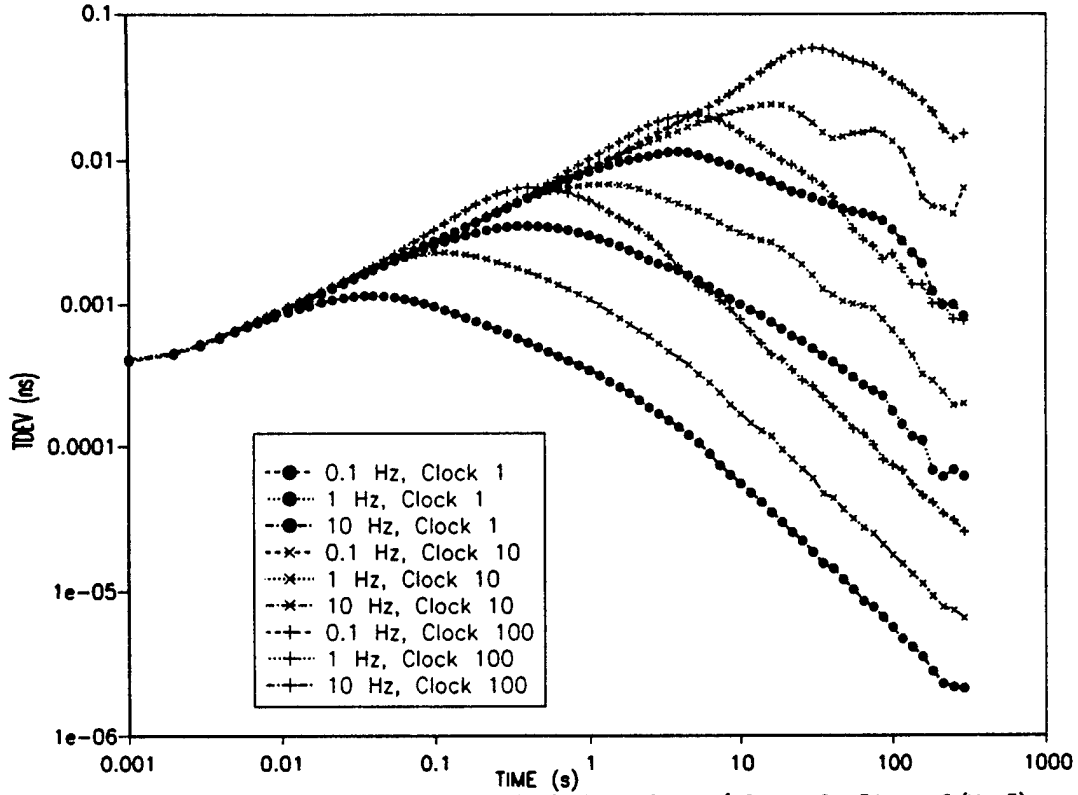
Figure 5. TDEV Due to VCO White FM Noise in Chain of Clocks ( b_0 = 4.0 \times 10^{-34} \text{ rad}^2/\text{Hz}^3 )
