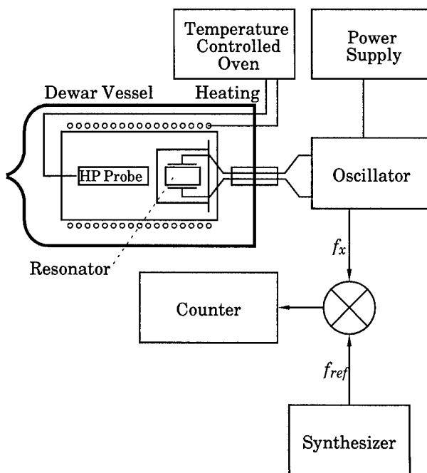
Fig. 13: Experimental setup
