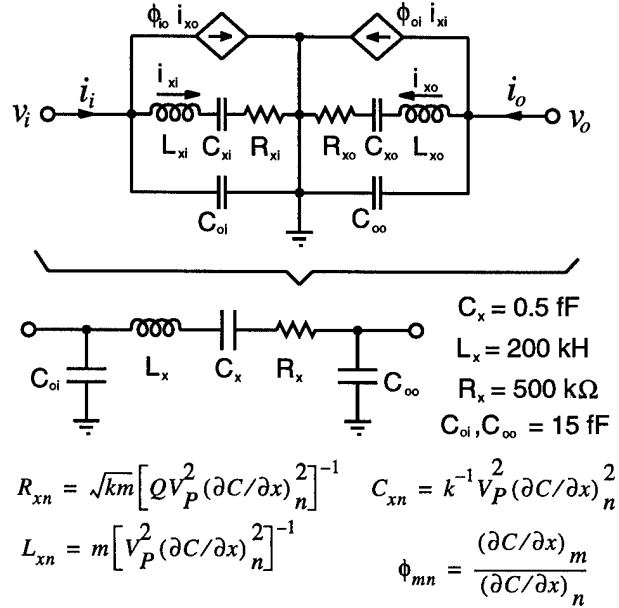
Fig. 6: Equivalent circuit for a two-port \mu resonator showing the transformation to the more convenient LCR form. In the equations, k is the system spring constant and (\partial C / \partial x)_n is the change in capacitance per displacement at port n of the \mu resonator.
