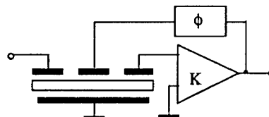
Fig. 2. Simple stage for BPF with active tuning.
