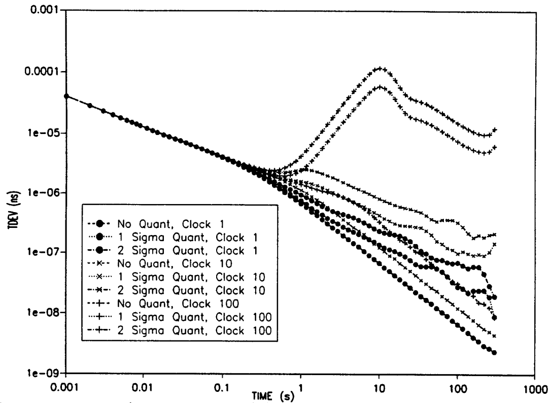
Figure 7. VCO White PM ( b_2 = 3.2 \times 10^{-16} \text{ rad}^2/\text{Hz} ), BW = 1 Hz, Quant in Multiple of VCO WPM Sigma
