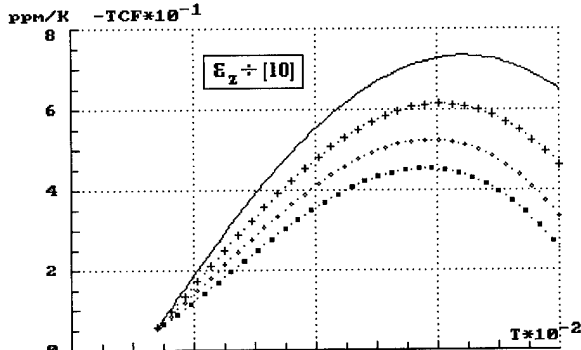
Fig. 2. Sapphire DDR TCF(T).
