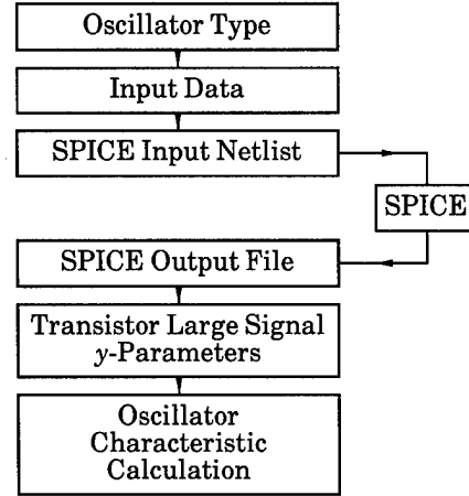
Fig. 9 : General flow chart of the program
