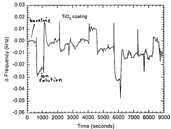
Figure 2. Plot of the sensor response to metal ion solutions
