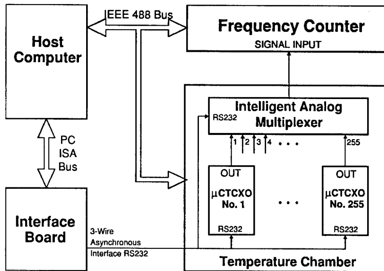
Fig.2 ACCL system.
