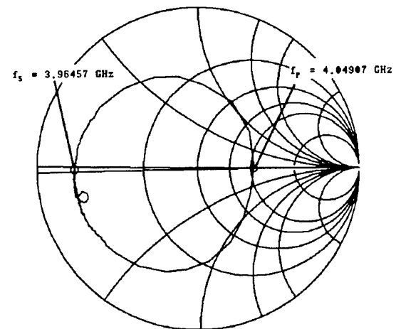
Fig. 3. S_{11} device measurement with k_t^2 > 5\%
