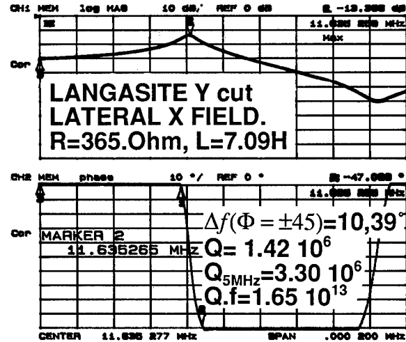
Figure 15: Response curves for a Y-cut LGS plano-convexe resonator showing an extremely large Q.f product at the resonance of the 7th overtone of the A mode (x field excitation).
