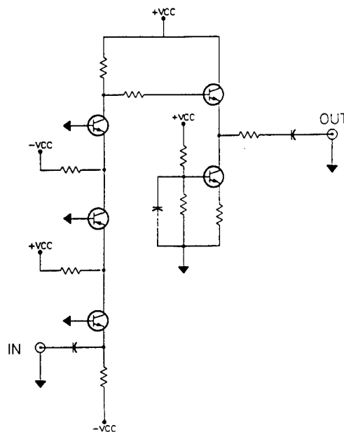
Figure 3. NIST's new isolation amplifier
