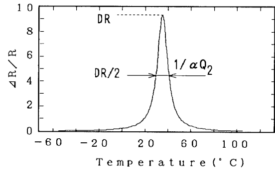
Fig.6 Meaning of Q_2 , DR and \alpha in a CI chart.
