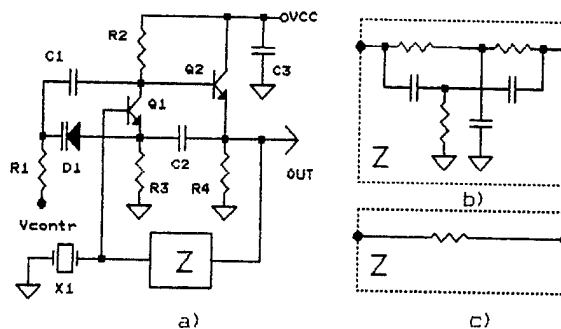
Fig. 16. The two-transistors dual-frequency oscillator network.
