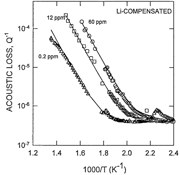
Figure 5. This \log(Q^{-1}) vs 1000/T plot shows that the high temperature acoustic loss for the Li-compensated samples is thermally activated.
