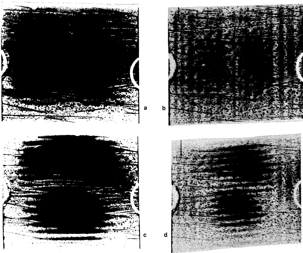
Figure 9-Topographs of the two antisymmetrical enharmonic modes. a and c/ the u_1 component. b and d/ the u_3 component.
