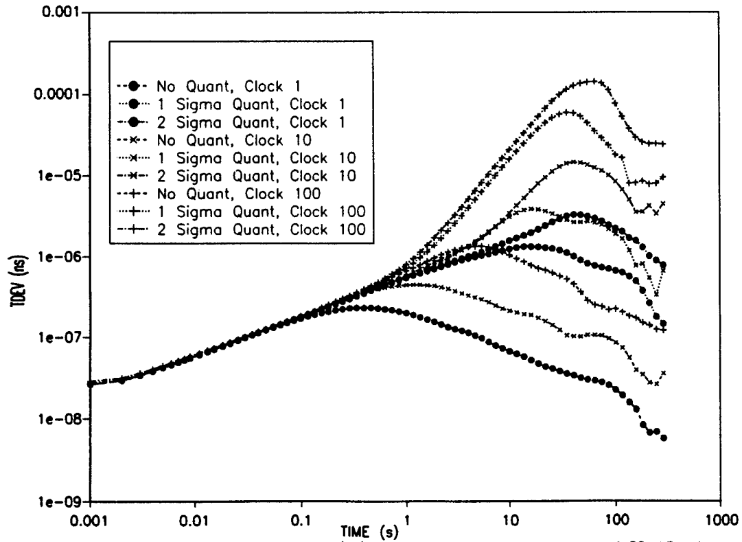
Figure 6. PD White PM ( c_2 = 1.0 \times 10^{-17} \text{ rad}^2/\text{Hz} , \text{BW} = 1 \text{ Hz} , Quant in Multiple of PD WPM Sigma)
