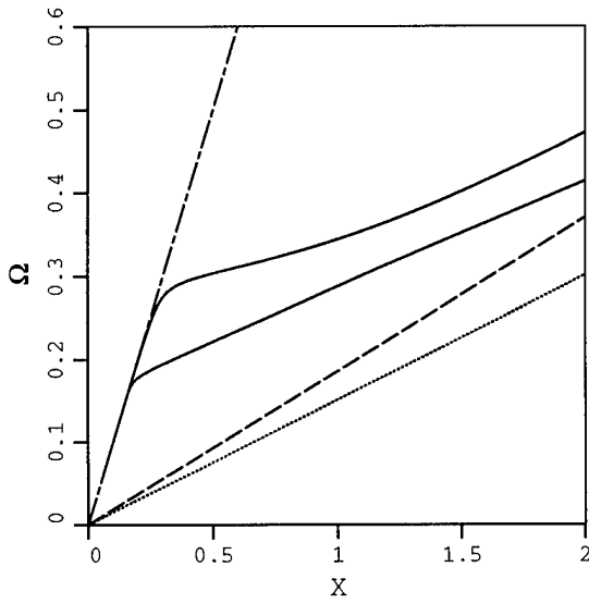
Figure 3: The second pair of dispersion curves for guided EM waves in a dielectric plate defined by (43), according to the 2-D equations.
