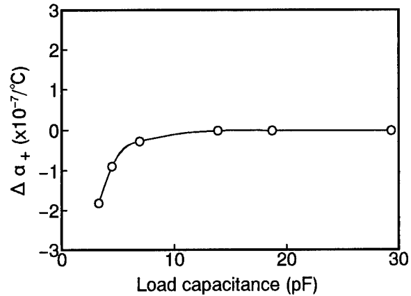
Figure 5. The variation of the first order frequency temperature coefficient of an NS-GT cut resonator ( \Delta\alpha_+ ) versus load capacitance. Courtesy of Seiko Electronic Components Co.,Ltd.
