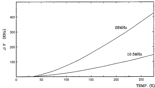
Frequency-Temperature Characteristics
