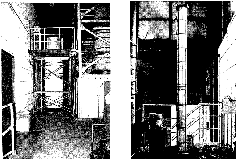
Figure 2. Photographs of the Autoclave and the Platinum Vessel with Iron Frame
