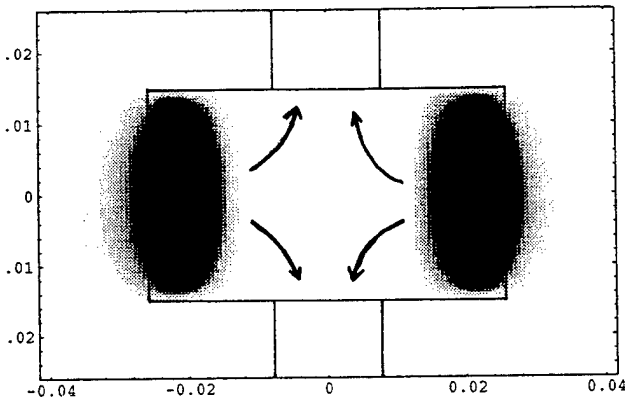
figure 7. Density plot of the axial electric field intensity of the E_{12\ 1\ \delta} mode in the axial plane of the resonator, dimensions are in \mu\text{m} . Arrows show the direction of heat flow.
