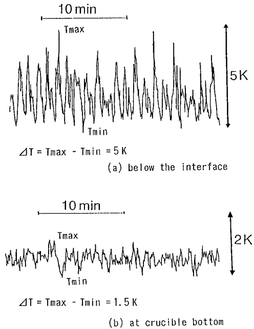
Fig.7. Typical examples of the temperature fluctuation. Crystal rotation rate is 0.3rpm.
