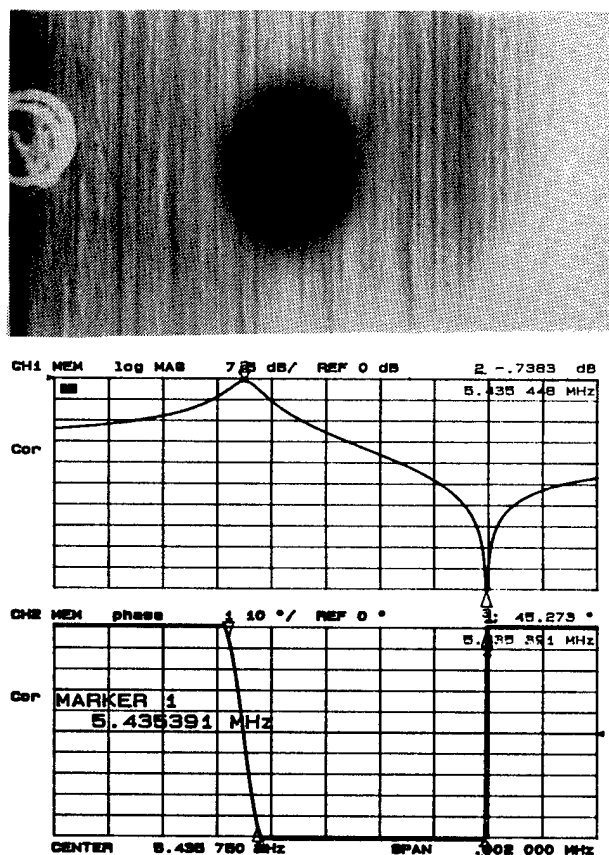
Figure 13-Topograph of the third overtone of the resonator represented in the figure 12b. The response curve shows a low transmission losses. We can remark that the phase slope is steep at the resonance but still more at the antiresonance.
