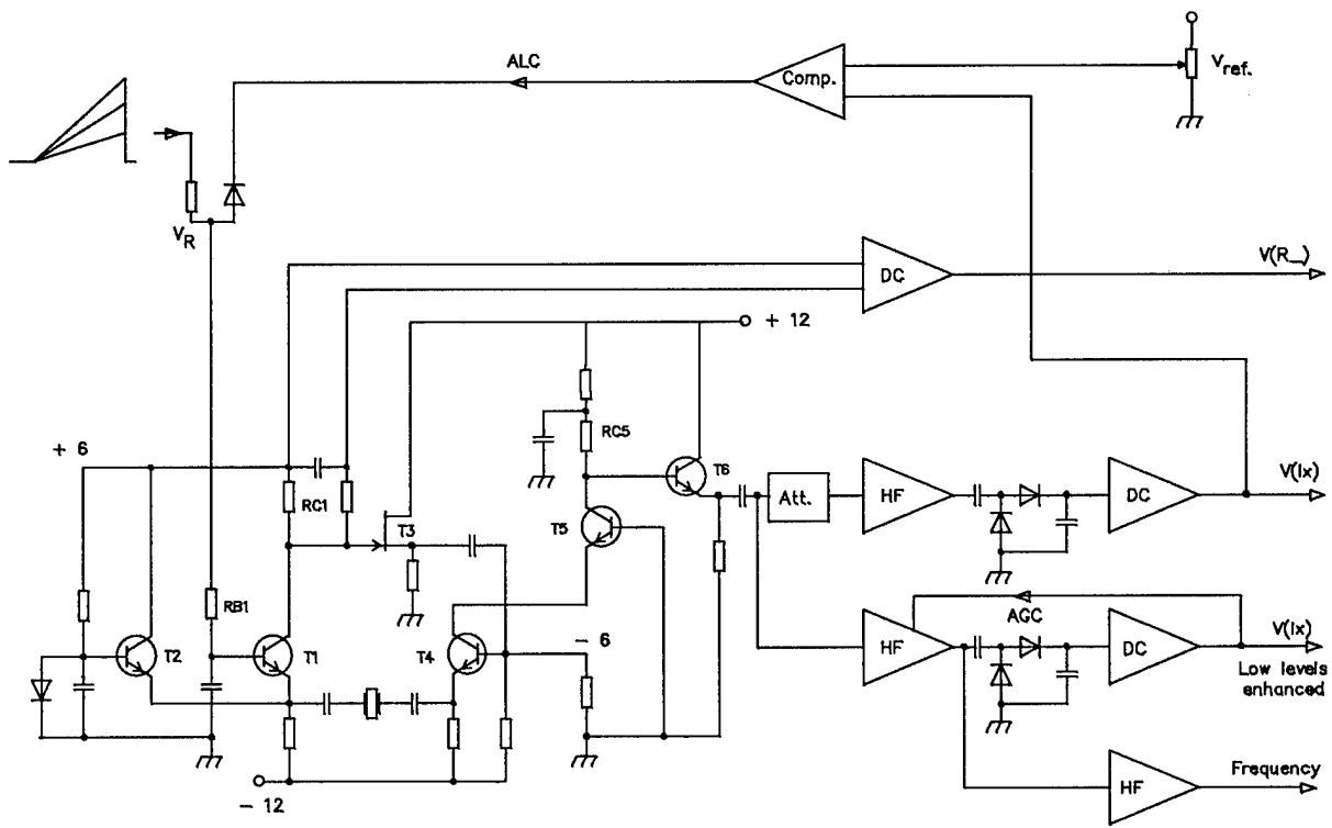
Fig.1 Schematics of the modified Butler-oscillator used for DLD characterisation of crystal resonators.
