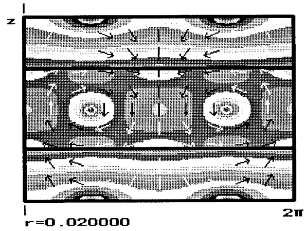
Figure 4.f: Electric (E) WGH 411 mode z- \phi plane.
