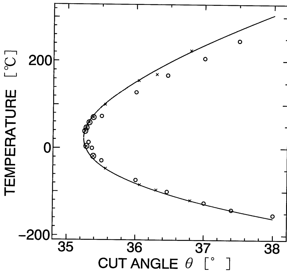
Fig.3. Frequency-turnover temperature vs angle of cut for the rotated Y-cut plate oscillating in c-mode in the vicinity of AT( x:present value, circle: BBL value 1,2) , cross - circle: value obtained by Koga and Shinada, solid line: quadratic curve of present.).
