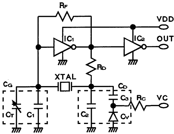
Figure 4. Circuit construction of the NS-GT-TCXO.
