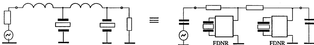
Fig. 9. Example of the filter circuit FDNR equivalent transformation
