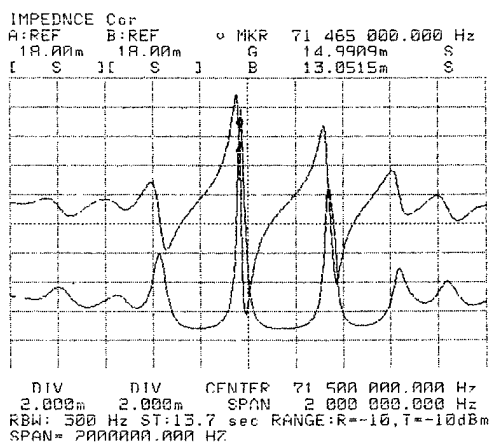
Fig.6. Wide-band response, IDTs in parallel.
