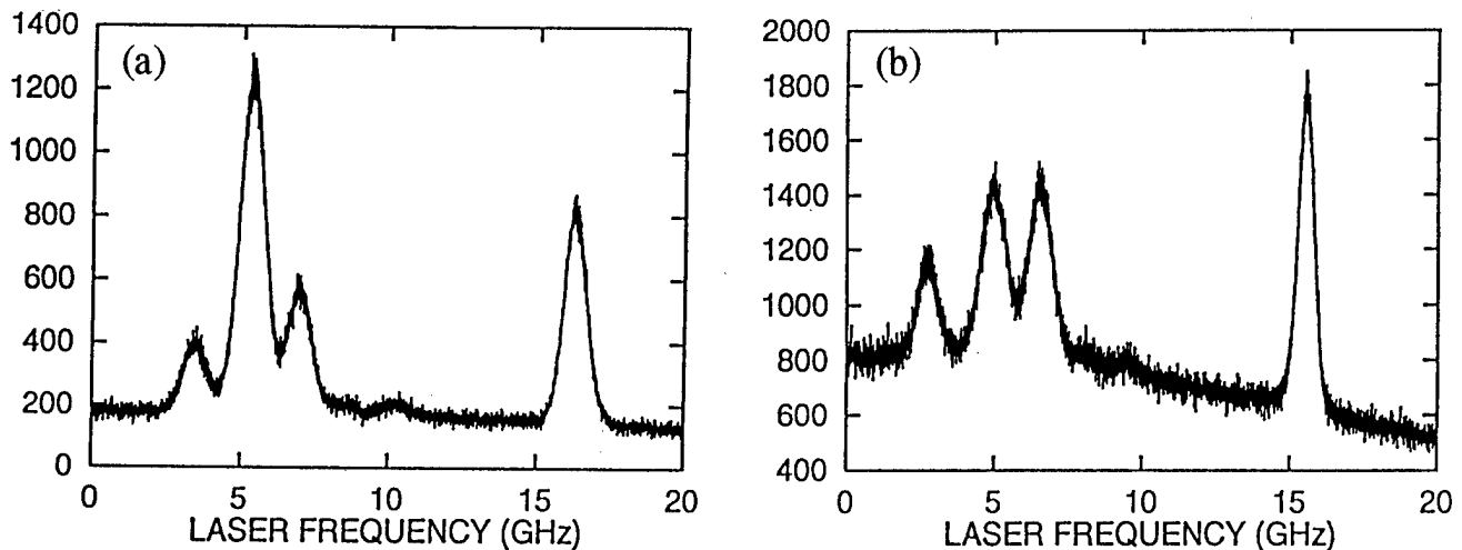
Figure 3: Resonance lineshape spectra vs. uv-laser power. (a) Laser power \sim 50 nW. (b) Laser power \sim 250 nW.
