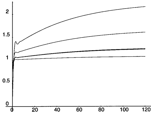
Figure 2: Average frequency uncertainty ratios for pure white phase noise ( \alpha = 2 ). Weighted least-squares fits to 31 points are extrapolated symmetrically from t_c to \tau . The standard uncertainty ratio to that for the unweighted fit (weights 'f') is plotted vs [\tau - t_c]/\Delta t . Weights 'a' (end points only) give the top curve (worst case), followed by weights 'b', 'c', 'd' and 'e'.
