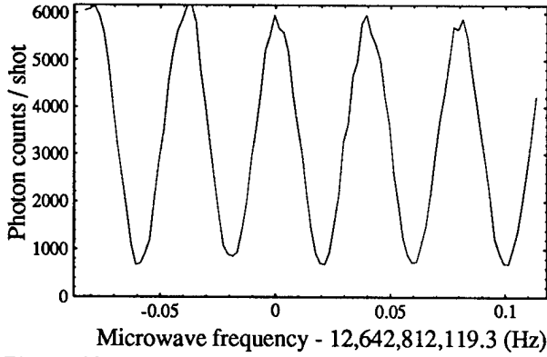
Figure 10: Ramsey fringes recorded using 25 s between microwave \pi/2 pulses. Each data point corresponds to a single pulse sequence. A background of 1500 counts / shot due to stray laser scatter has been subtracted. The noise and amplitude drift is primarily due to laser power fluctuations.
