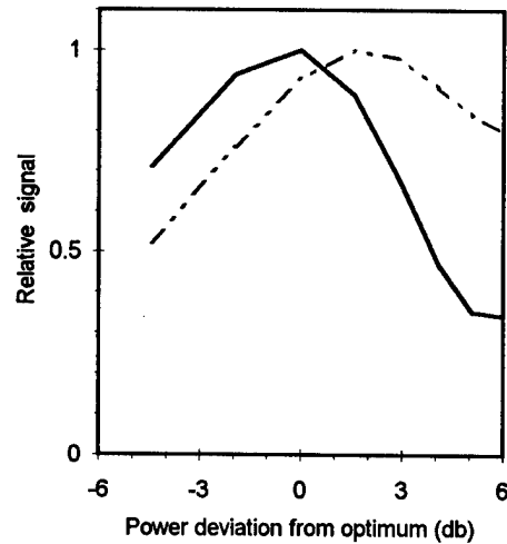
Figure 9: Dependency of the SHLM (full line) and the BCM (dashed line) on microwave power. Power is "optimized" for the peak of the speed distribution. The speed distribution shown in Fig. 5 was used in the calculations.
