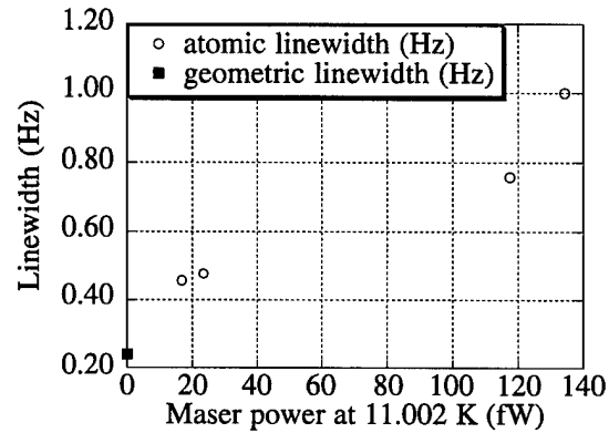
Figure 3. Maser power versus linewidth.
