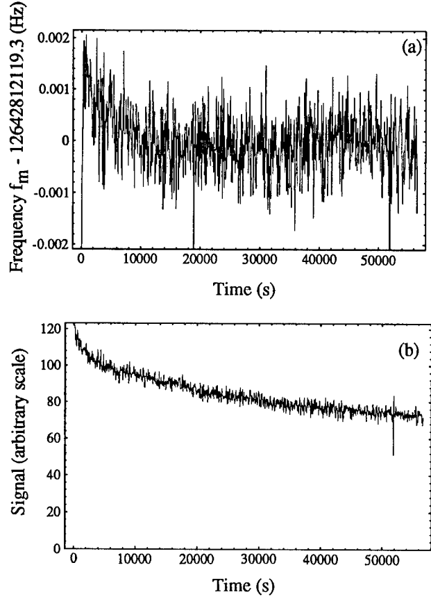
Figure 11: a) Measurement of the standard frequency f_m as a function of time. b) Variation of the signal from the ion trap (compensated for laser power drift) during the same measurement. The end electrode potential was 20 V.
