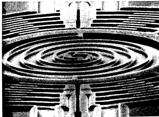
Figure 3. SEM of polysilicon torsional microresonator [12].
