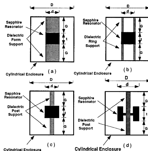
Fig. 1 Sapphire DR loaded cavity with (a) form support (b) ring support (c) post support (d) support structure for ring resonator.
