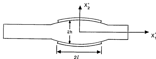
Figure 1 Cross-Section of a Biconvex Resonator
