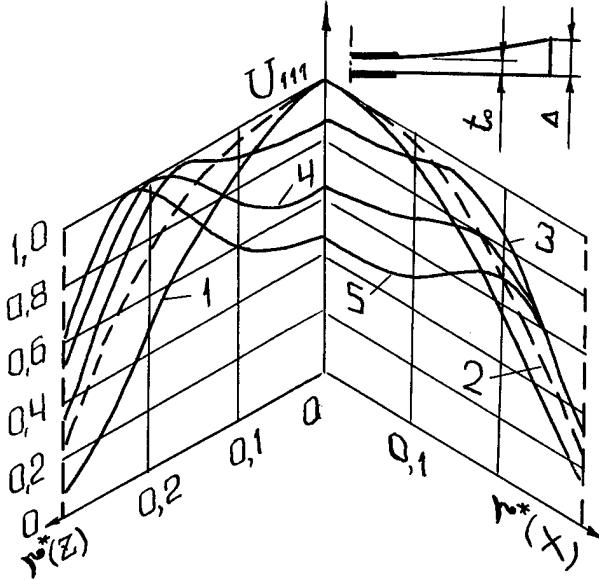
Figure 7 - Influence of PE concavity on displacement distributions at PE surface for the fundamental frequency ( d/t_0=200 ; d_e/d=0.3 ; te^*=0.035 ): 1 curve - \Delta/t_0=0 ; 2-0.03; 3-0.05; 4-0.07; 5-0.09.
