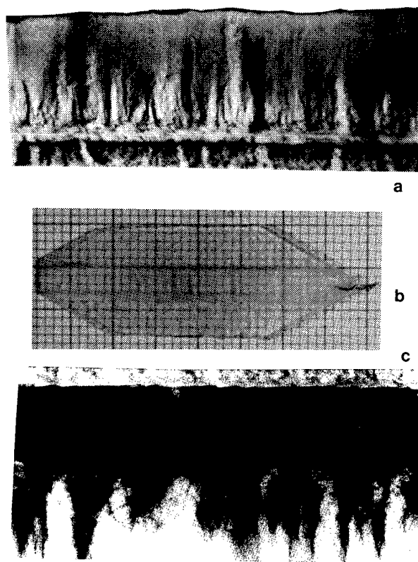
Figure 2 -This gallium phosphate crystal in b, obtained from a z berlinite seed in sulphuric acid and VTG method, has only the growth rate along X significant. In a and c two traverse topographs of this crystal.
