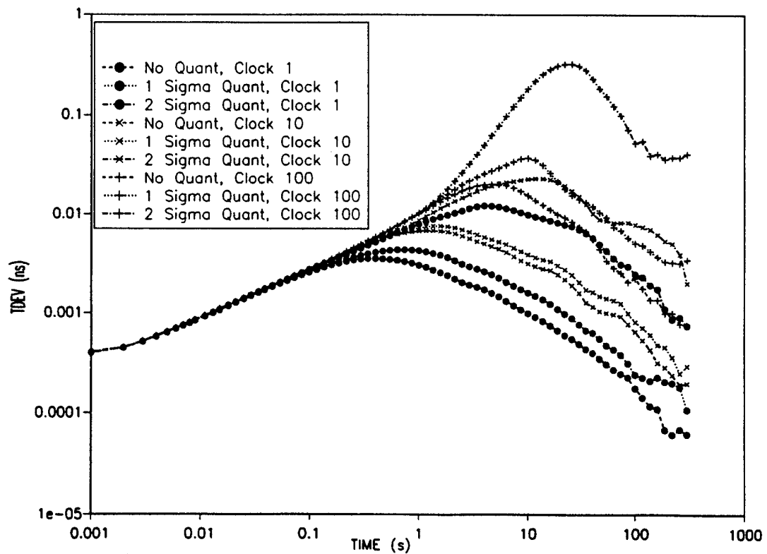
Figure 8. VCO WFM ( b_0 = 4.0 \times 10^{-34} \text{ rad}^2/\text{H}^3 ), BW = 1 Hz, Quant in Mult of VCO WFM Sigma at 5.6 ms
