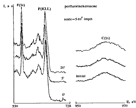
Fig.15. XPS spectra for PPC from perfluorinckerosene e-irradiated in the same conditions as it is indicated in Fig.14.
