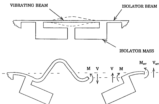
FIGURE 2 VIBRATION ISOLATOR TO MAINTAIN HIGH Q
