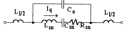
Figure 2. Circuit model of a crystal resonator
